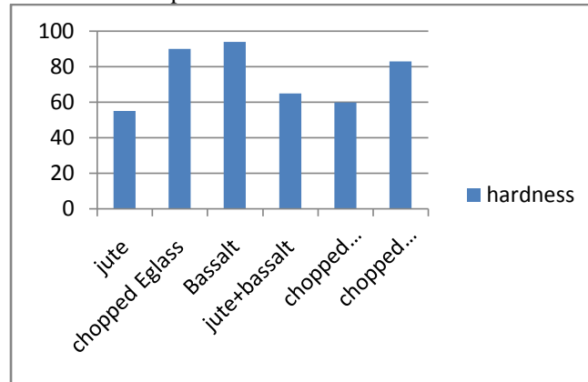
Figure 8: Hardness comparison Graph
