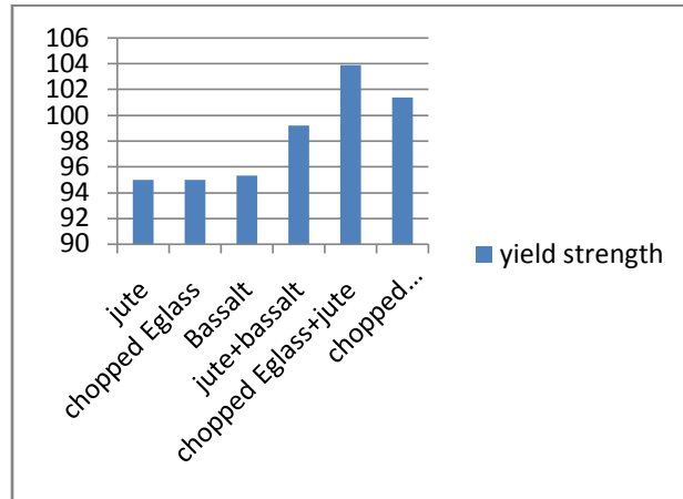
Fig 5: yield strength comparison graph.
