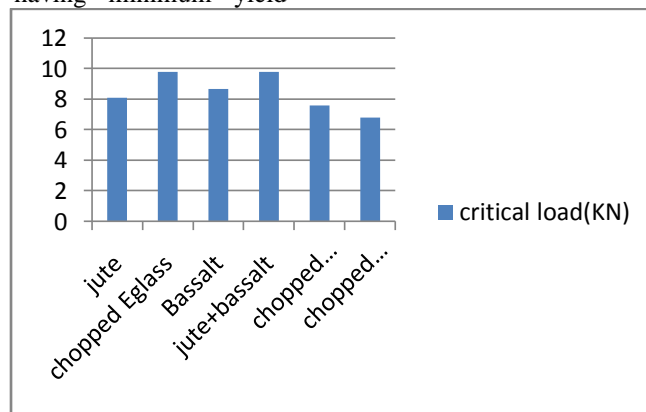
Fig 6: critical load comparison graph.
